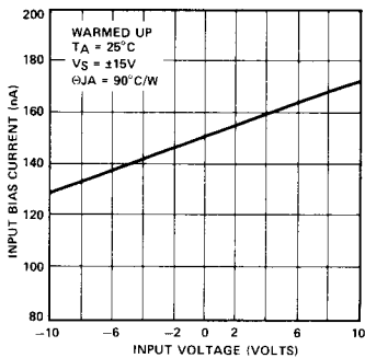
INPUT BIAS CURRENT vs INPUT VOLTAGE
